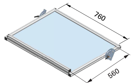
Adjustable shelf with tilt brackets Frame - 30x30 and 30x60 profile Board - 8mm melamine board
