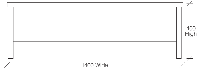
LOMCOFF01 – 1400W x 700D x 400H | Shelf
