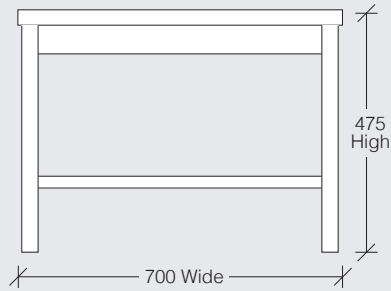
LOMLAM01 – 700W x 700D x 475H | Shelf
