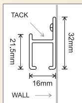
The Gallery System Track
