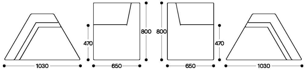
CORNER SEAT WITH BACK (LEFT AND RIGHT SIDED)
