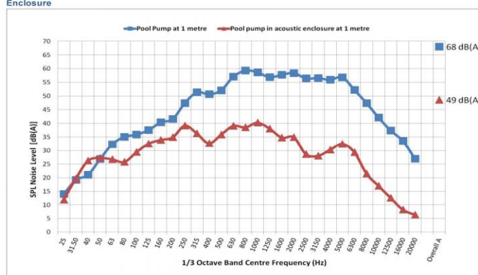
Figure 6.1 Overall A-Weighted & 1/3 Octave Band Noise Levels - Pool Pump With and Without Acoustic Enclosure
