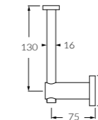
Spare toilet roll holder 2262931
