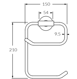
Double stirrup toilet roll holder 225935
